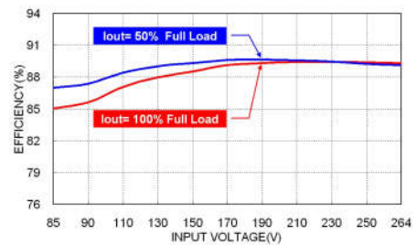
TSD30US24B Efficiency vs. Input Voltage
