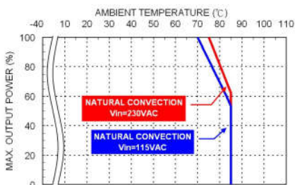
Derating Curve vs. Ambient Temperature TSD30USxxB xx=12/15/24/28/36/48/53 Connector Option : (Blank: JST)
