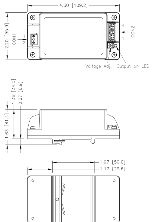
BOTTOM VIEW
